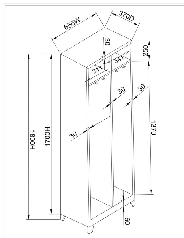
Internal dimensions
