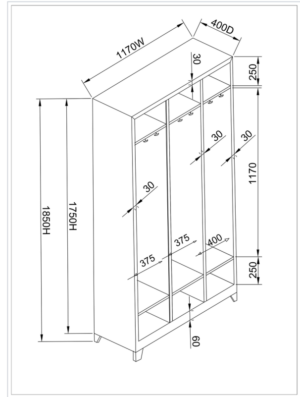
Internal dimensions
