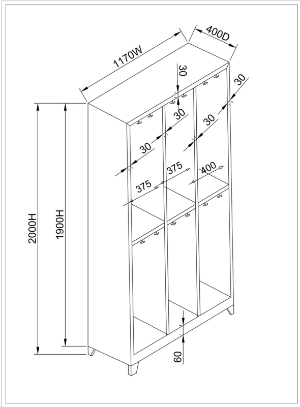
Internal dimensions
