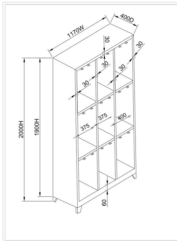
Internal dimensions
