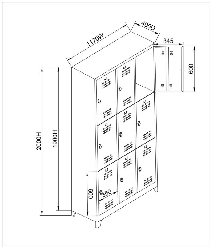
Exterior view
