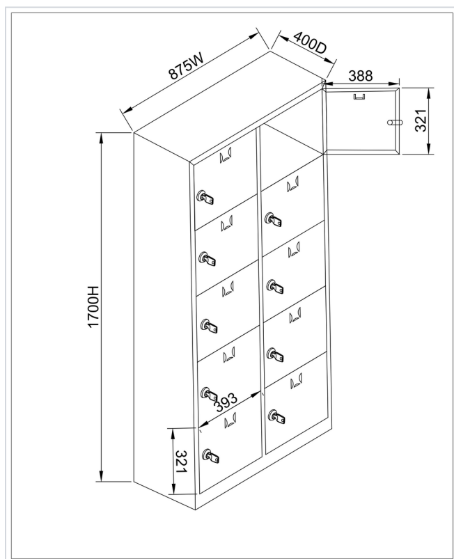
Exterior view
