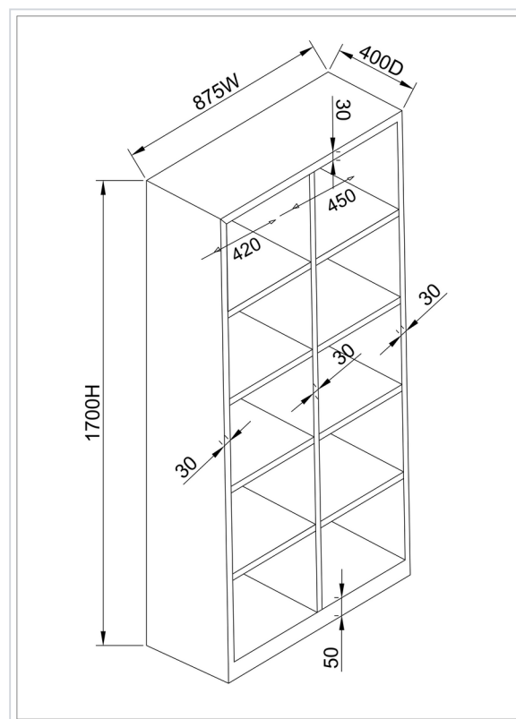
Internal dimensions
