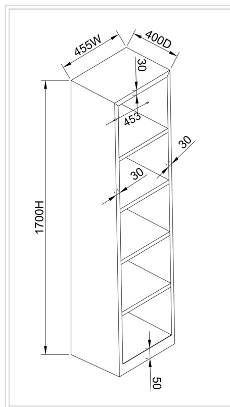
Internal dimensions
