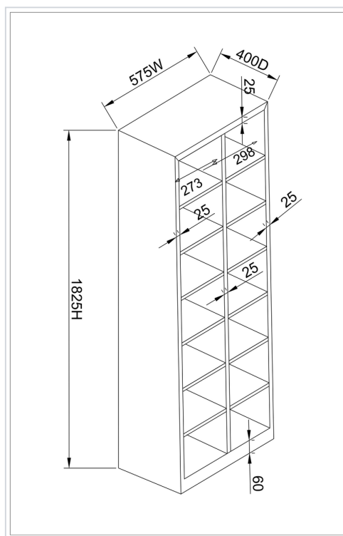
Internal dimensions
