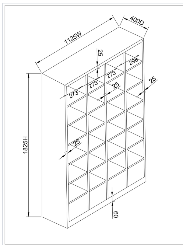
Internal dimensions
