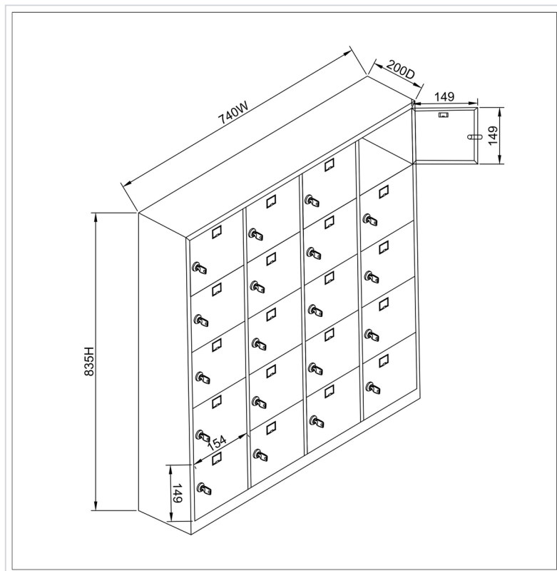
Exterior view
