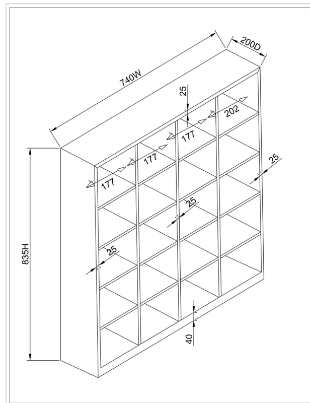
Internal dimensions
