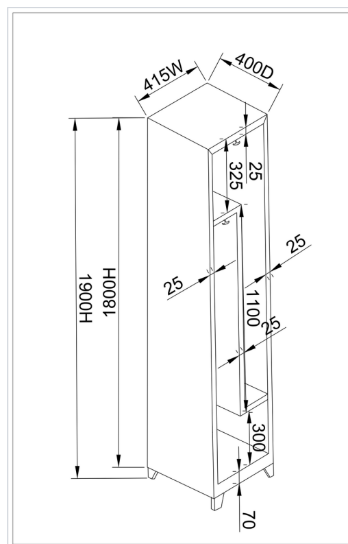
Internal dimensions
