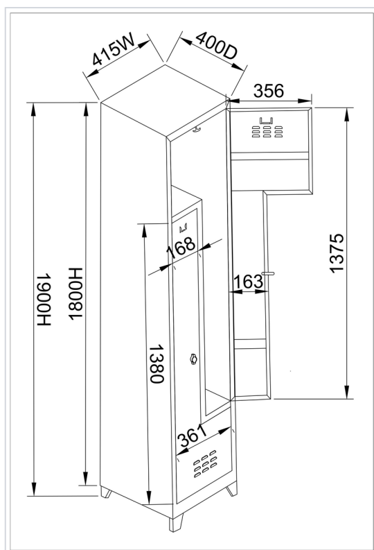
Exterior view
