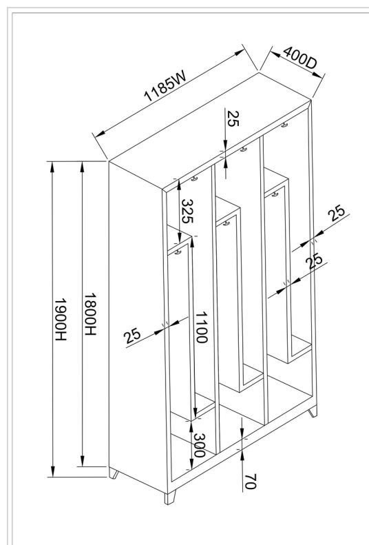
Internal dimensions
